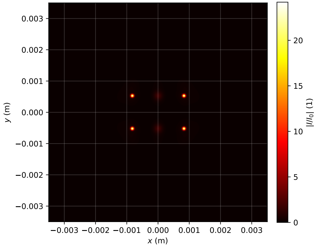
Intensity profile I(x, y, z = 0.478)/I_0 , P_{in}=9.0P_{cr} , artificial time
